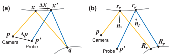
Fig. 7. The geometry of path perturbations. (a) From a known specular path ( q, x, p ) and a probe position p' , a new path ( q, x', p' ) can be determined through local path perturbation. (b) To assess probe samples, we compute a score based on ray information (reflector and reflected positions, reflector normal) associated with the sample ( r_p, n_p and R_p ) and the novel view pixel ( r_v, n_v and R_v ).
