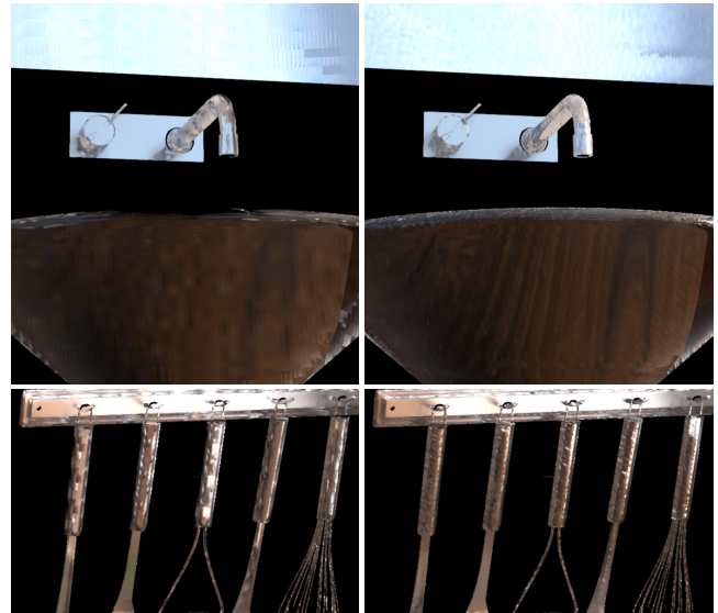
Fig. 12. Comparing (left) regular and (right) our adaptive parameterization when warping just a single probe into the novel view. Top: Bathroom scene, Bottom: Small Kitchen. For clarity, we do not apply our glossiness filter.
