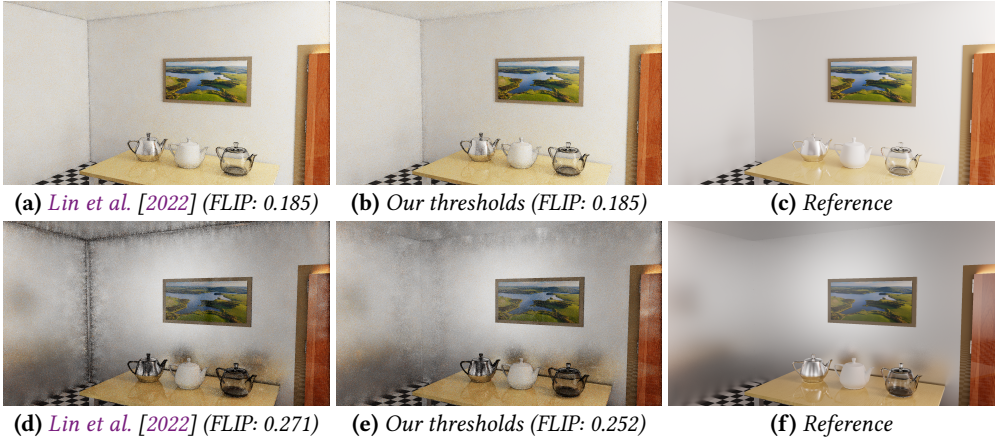
Fig. 12. Lin et al.’s [2022] reconnections perform similarly to our work in diffuse scenes like VEACH AJAR. With metallic walls (roughness of 0.3), their baseline shows significantly more noise. Our new thresholds automatically enlarge reconnection distances, giving more consistent noise.
