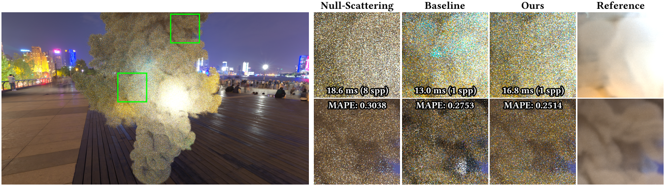
Figure 2: Highly anisotropic static PLUME volume ( g = -0.95 ) lit by a high-contrast SHANGHAI environment map, with near equal-time comparison. Baseline cannot use MIS between NEE and phase-sampled paths, leading to severe correlation artifacts. Our formulation enables technique MIS, substantially reducing both noise and correlation compared to Null-Scattering and Baseline . The scene is captured under camera motion.
