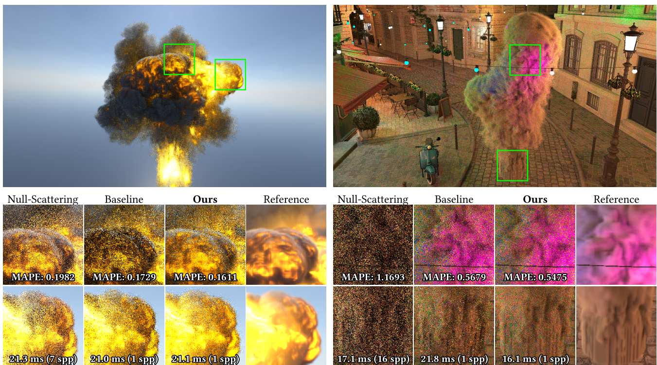
Figure 1: Ghost ReSTIR improves both quality and performance over null-scattering path tracing [Galtier et al. 2013; Miller et al. 2019] and prior volumetric ReSTIR [Lin et al. 2021]. (Left) EXPLOSION , a dense emissive volume under 9-bounce multiple scattering and dynamic camera—prior volumetric ReSTIR shows severe noise in dense emissive regions from its inconsistent \hat{p} , which our consistent formulation substantially reduces. (Right) BISTRO , a smoke plume lit by many colored area lights and surfaces in single scattering—ours handles volume–surface interaction more cleanly and runs 1.4× faster thanks to null-scattering tracking that avoids the costly voxel traversal of regular tracking.
